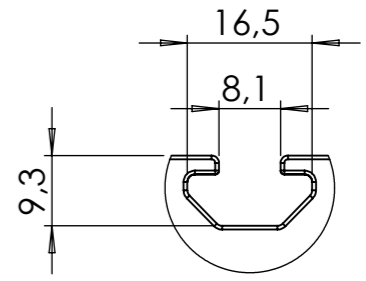
DETAIL A Type 30 - T-slot SCALE 1 : 1
