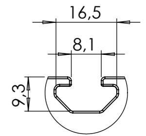
DETAIL A Type 30 - T-slot SCALE 1 : 1
